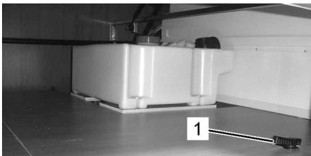
Abb. 104: Ablasshahn (1)
